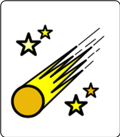
comet/fireball
