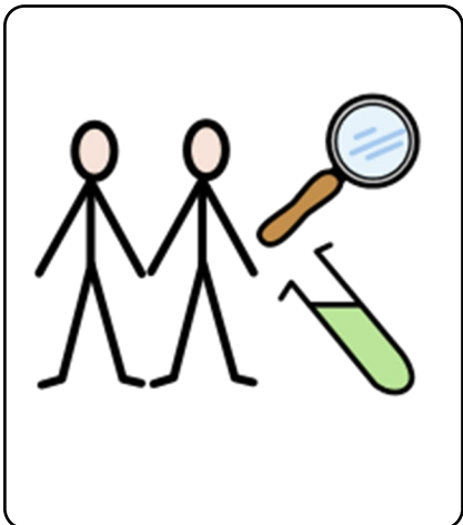
scientists
