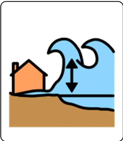
tsunami
